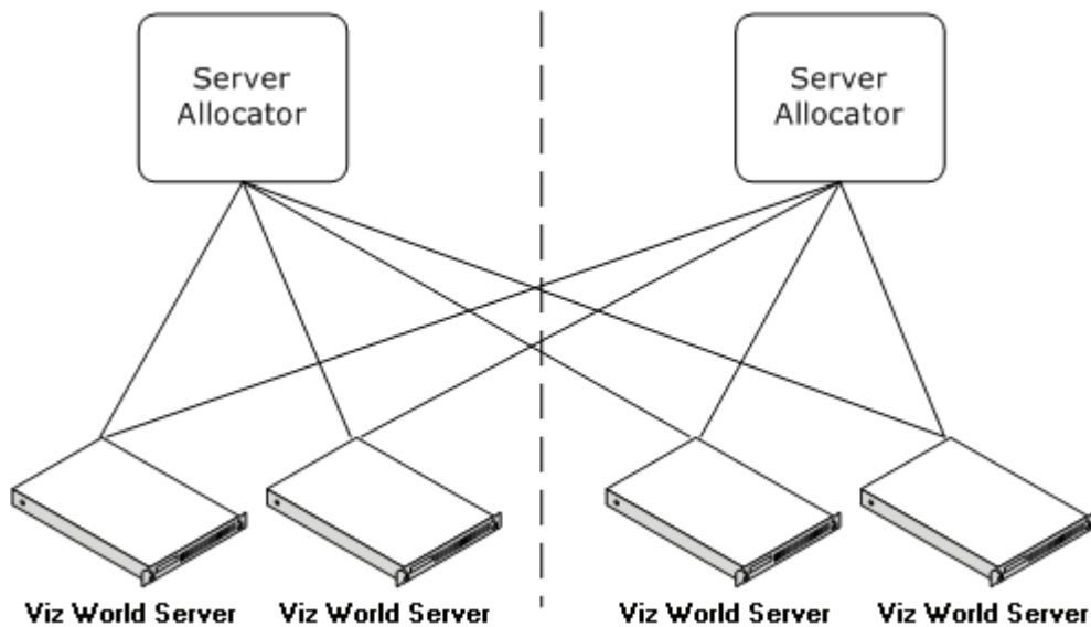
Figure 21: Multiple Server Allocators with Multiple Map Servers.
