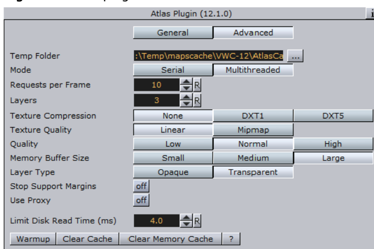
Figure 74: Atlas plugin Advanced tab
