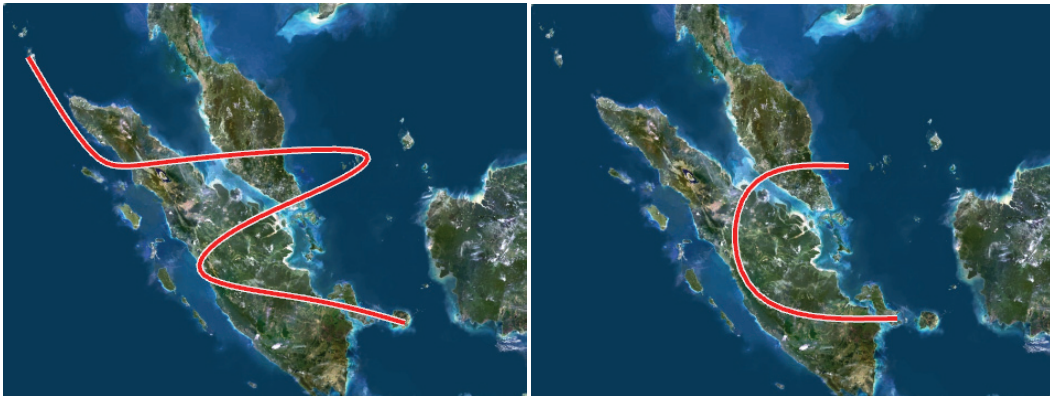
Figure 93: Control points
