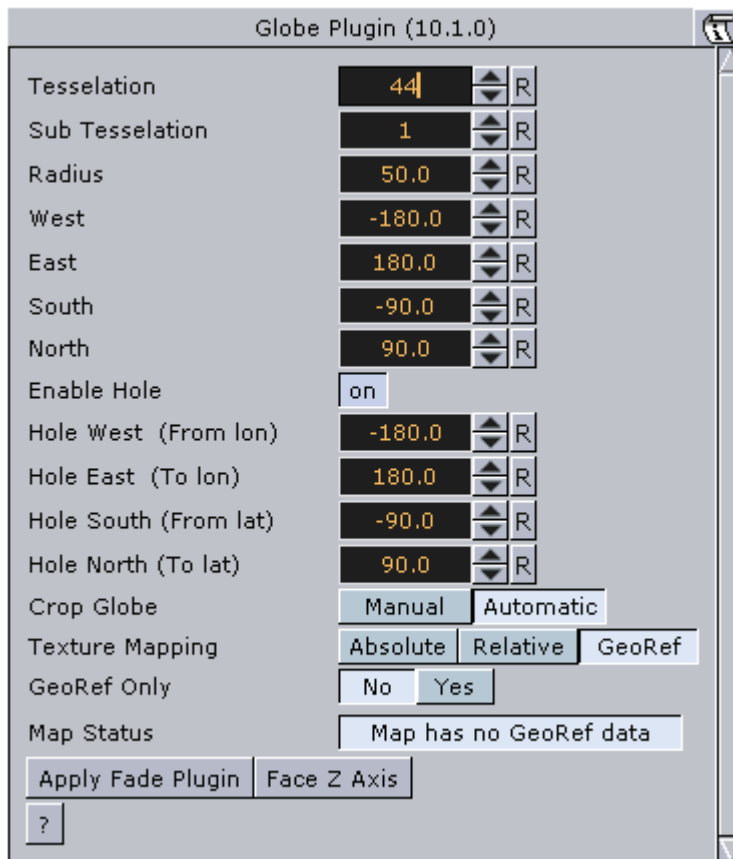
Figure 82: Globe editor
