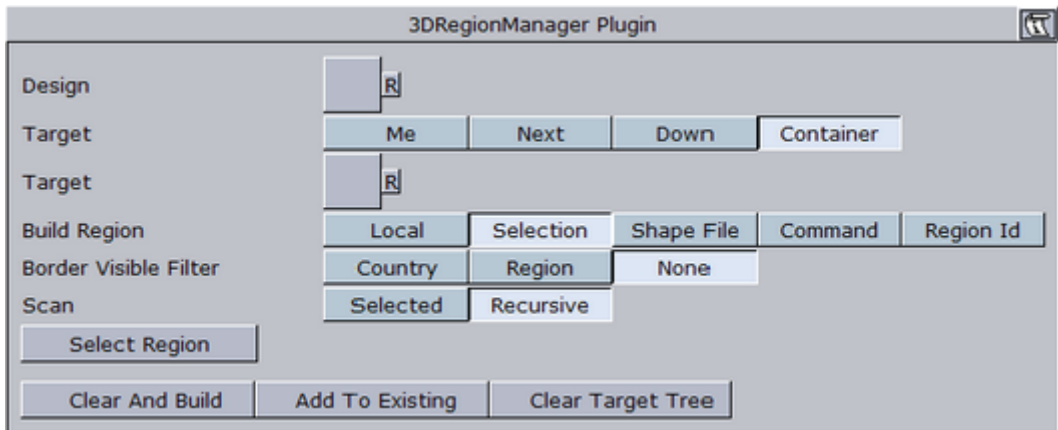
Figure 100: Target set to Container, 3D Region Manager editor
