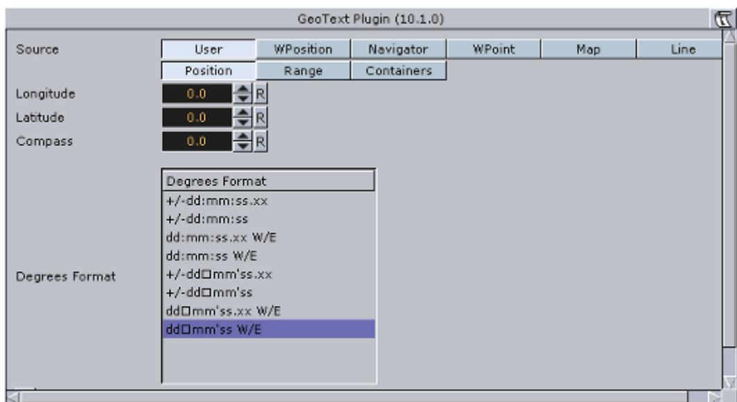
Figure 127: Source set to User and Position, Focus On Map editor
