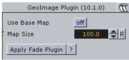
Figure 78: Geolmage editor
