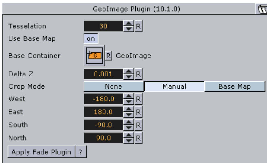
Figure 80: Crop Lon/Lat, GeoImage editor
