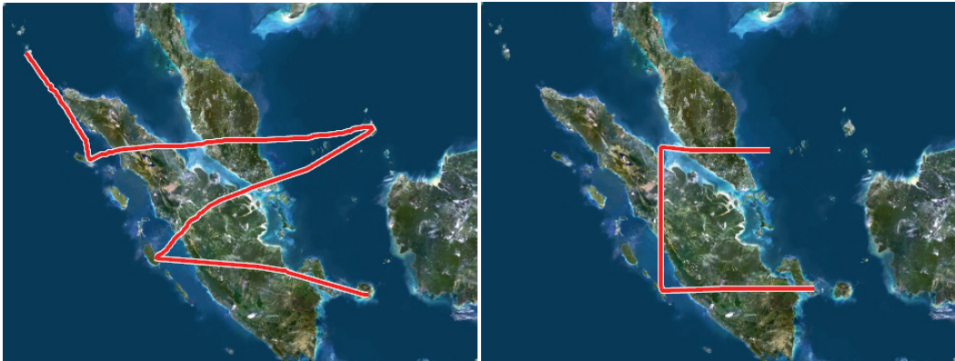
Figure 92: Original curves
