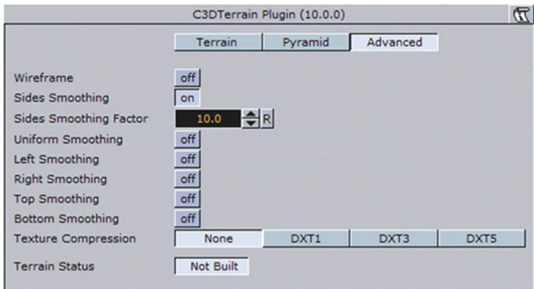
Figure 109: Advanced, Curious 3D Terrain editor
