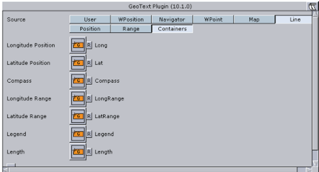
Figure 129: Source set to User and Containers, Focus On Map editor
