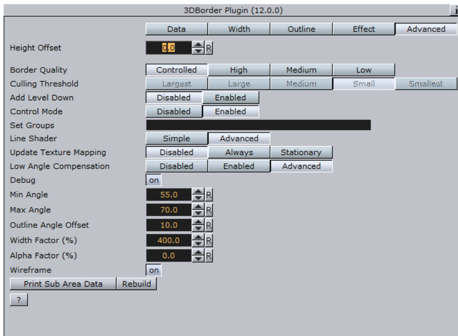
Figure 44: Advanced, 3D Border editor
