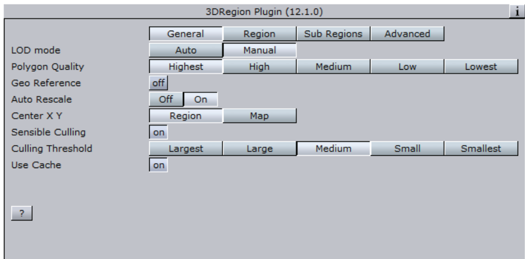
Figure 58: General, 3D Region editor
