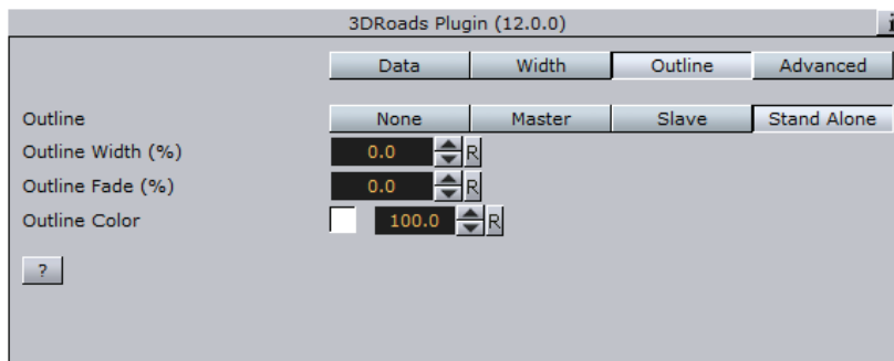
Figure 72: Outline, 3D Roads editor
