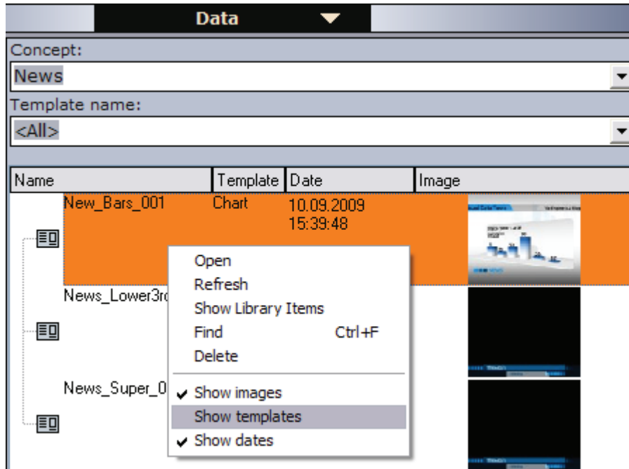
Figure 64: Data resources
