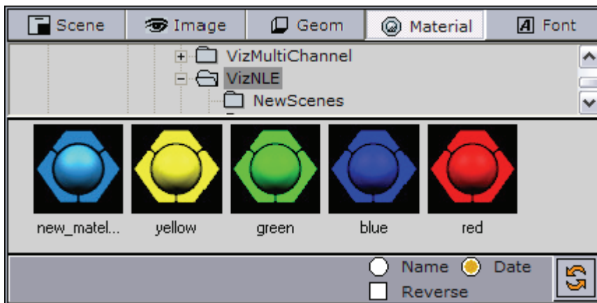
Figure 70: Materials
