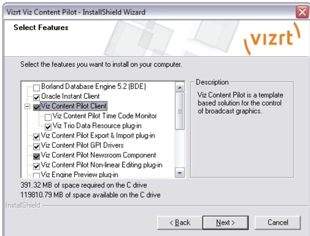
Figure 9: Select Features
