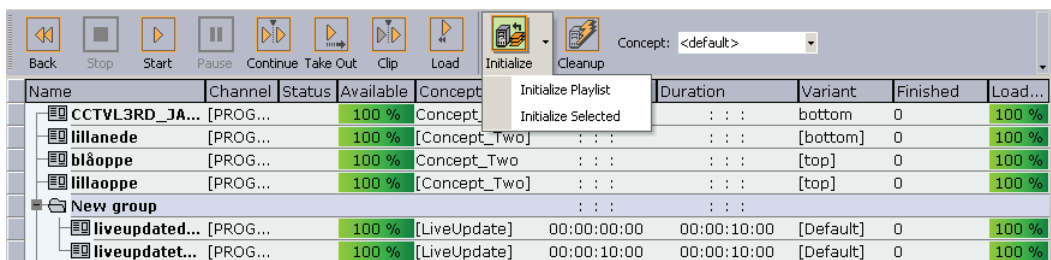
Figure 79: Item toolbar
