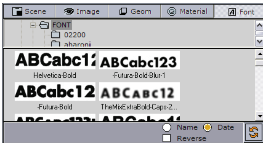
Figure 71: Fonts
