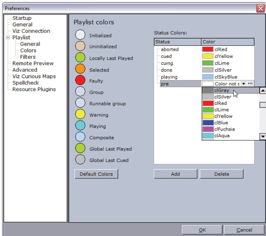
Figure 39: Playlist colors
