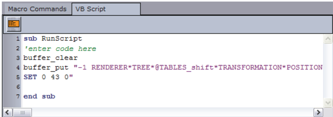
Figure 33: VB Script
