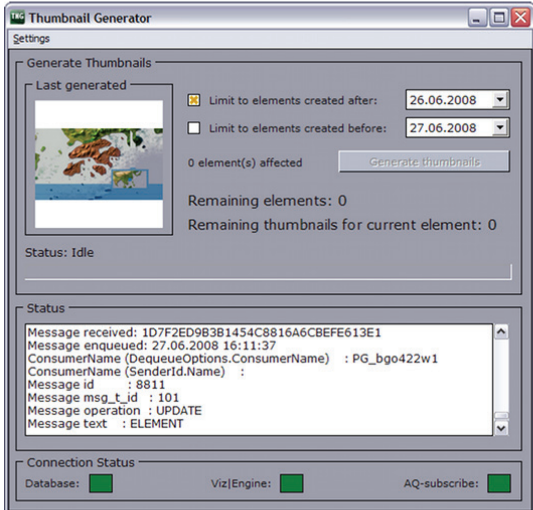
Figure 99: User interface
