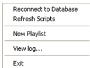
Figure 27: File menu
