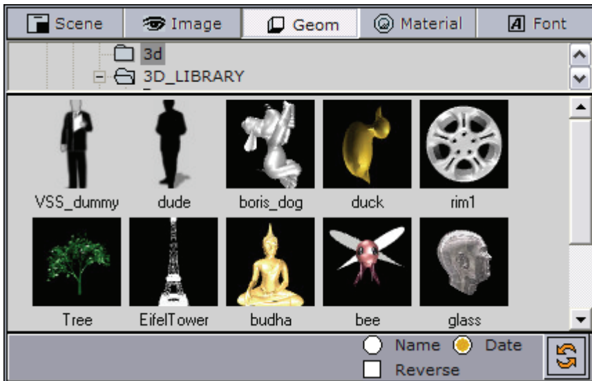
Figure 69: Geometry objects
