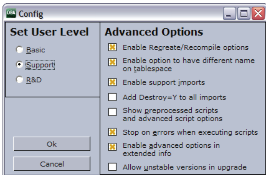
Figure 103: Advanced Configuration
