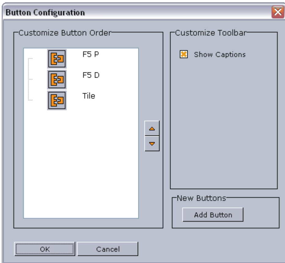
Figure 81: Button Configuration
