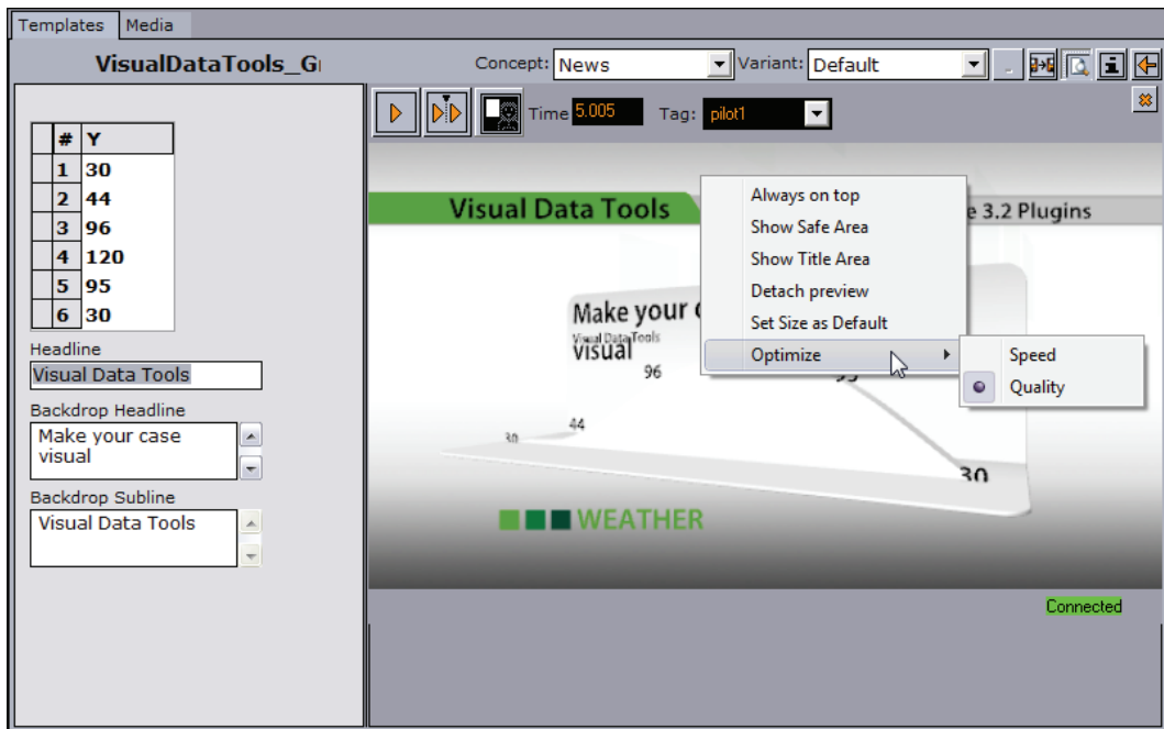
Figure 91: Saved data element with remote preview enabled
