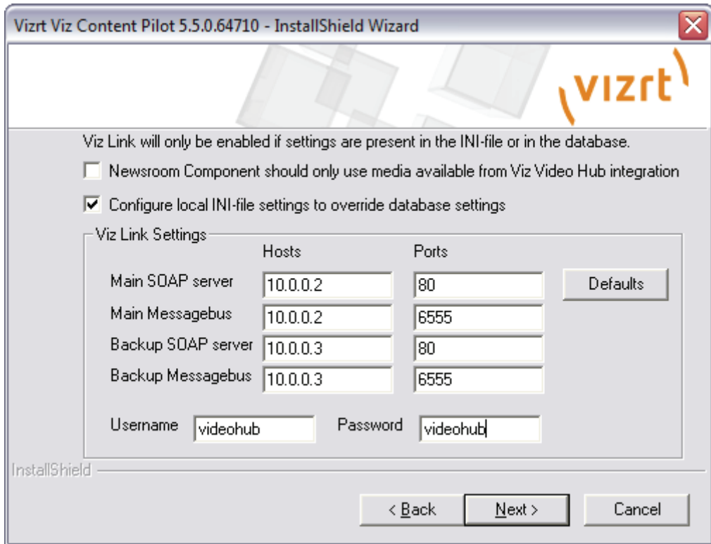
Figure 6: Viz Link configuration
