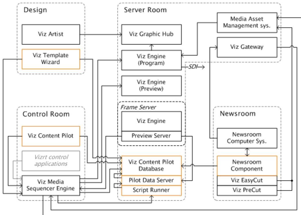
Figure 1: VCP system overview
