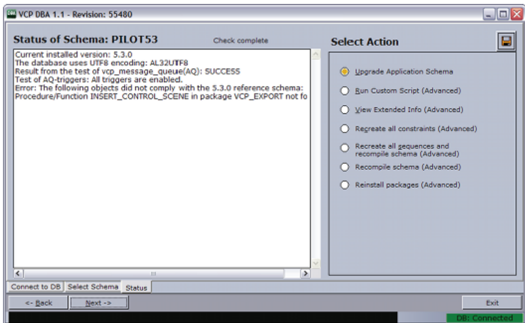
Figure 104: Status of schema
