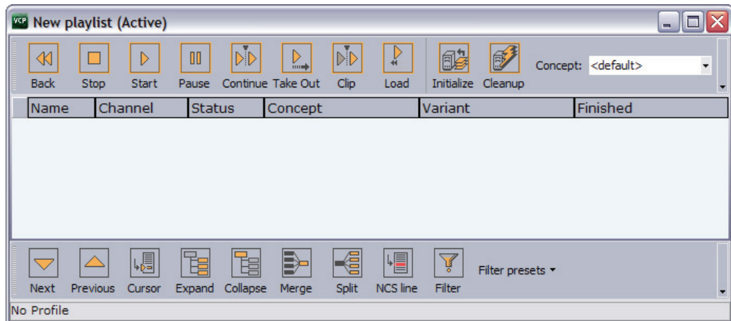
Figure 78: Playlist
