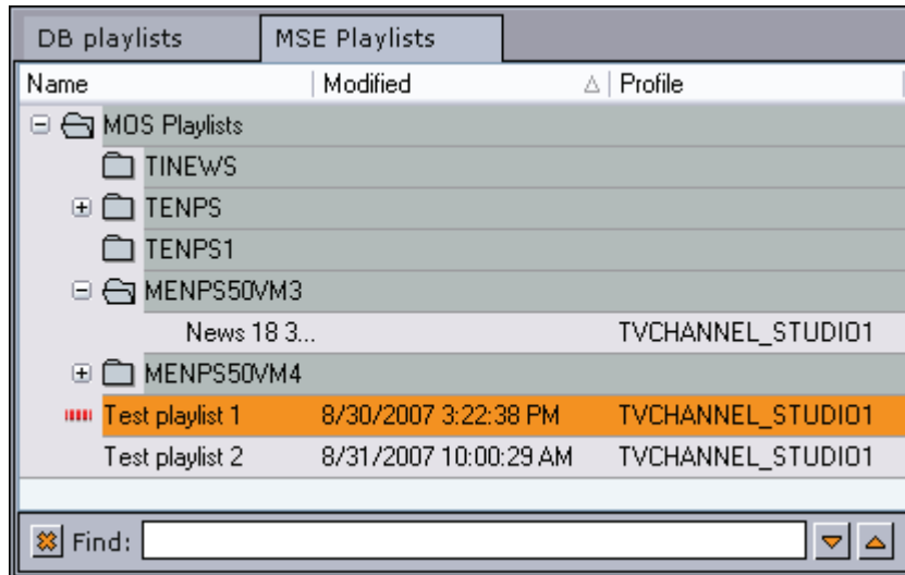
Figure 65: Playlist resources
