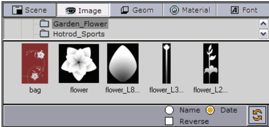
Figure 68: Images
