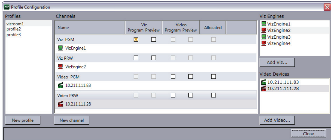
Figure 10: Profile Configuration
