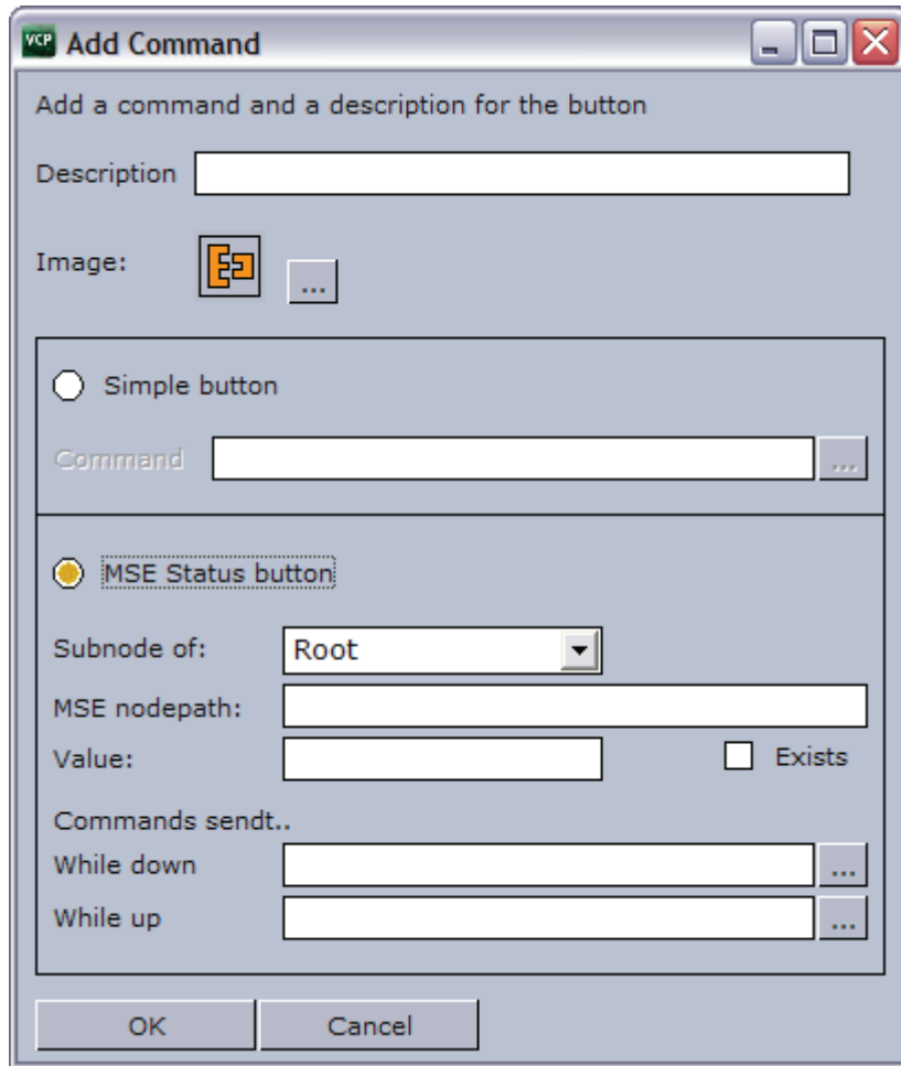
Figure 82: Add Command
