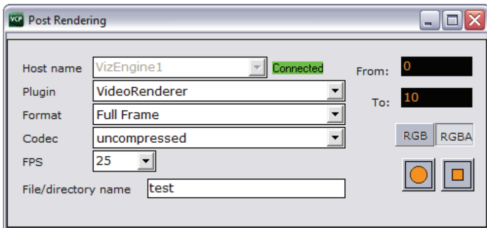
Figure 52: Post rendering
