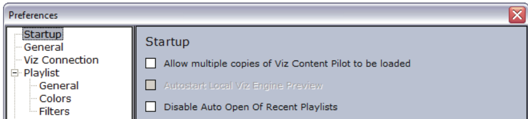
Figure 35: Startup
