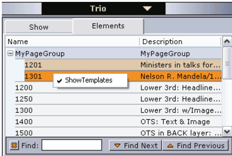
Figure 75: Elements view
