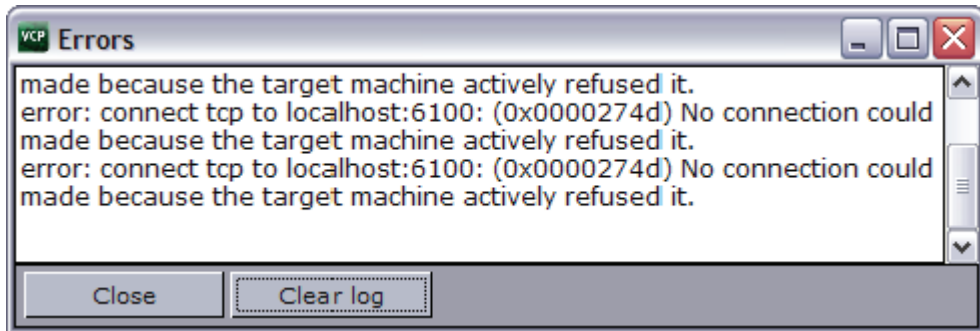
Figure 61: Error log
