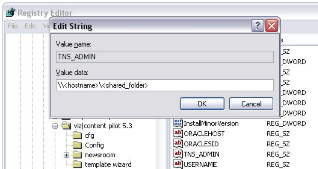
Figure 19: Registry setting
