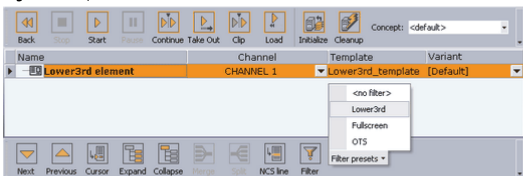
Figure 42: Playlist filtered
