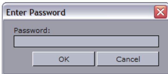
Figure 55: Enter Password
