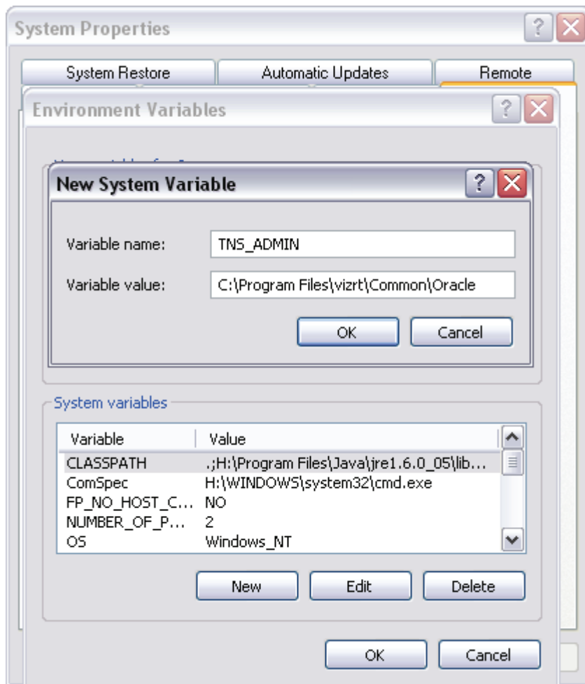
Figure 20: Environment variable
