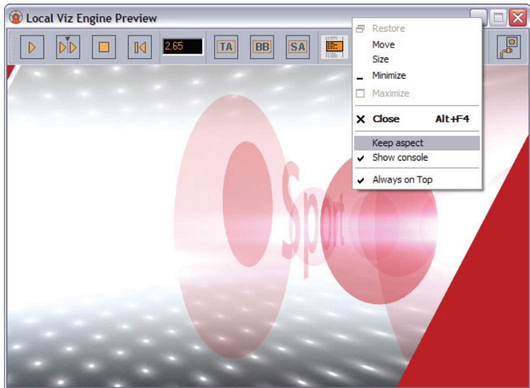
Figure 56: Local preview
