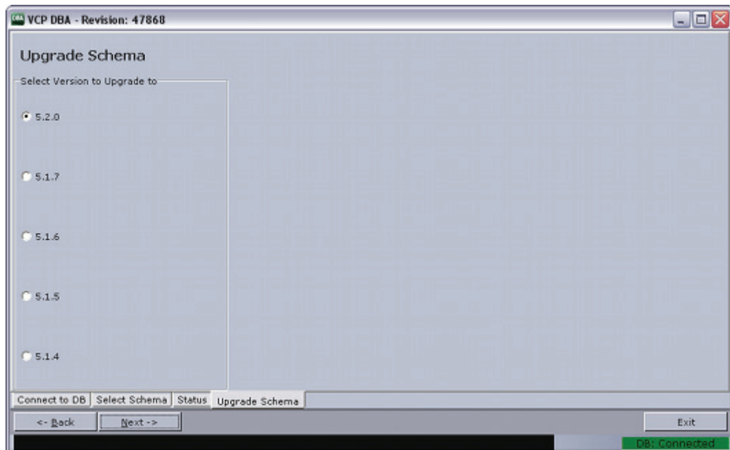
Figure 107: Upgrade schema
