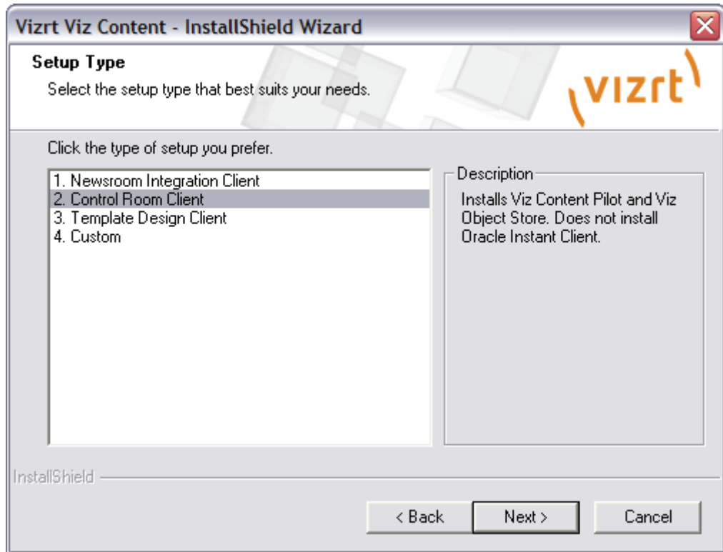
Figure 2: Setup Type
