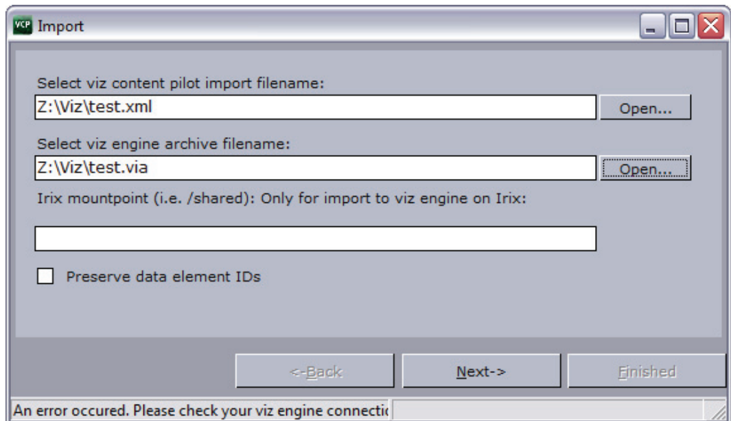
Figure 50: Import playlist
