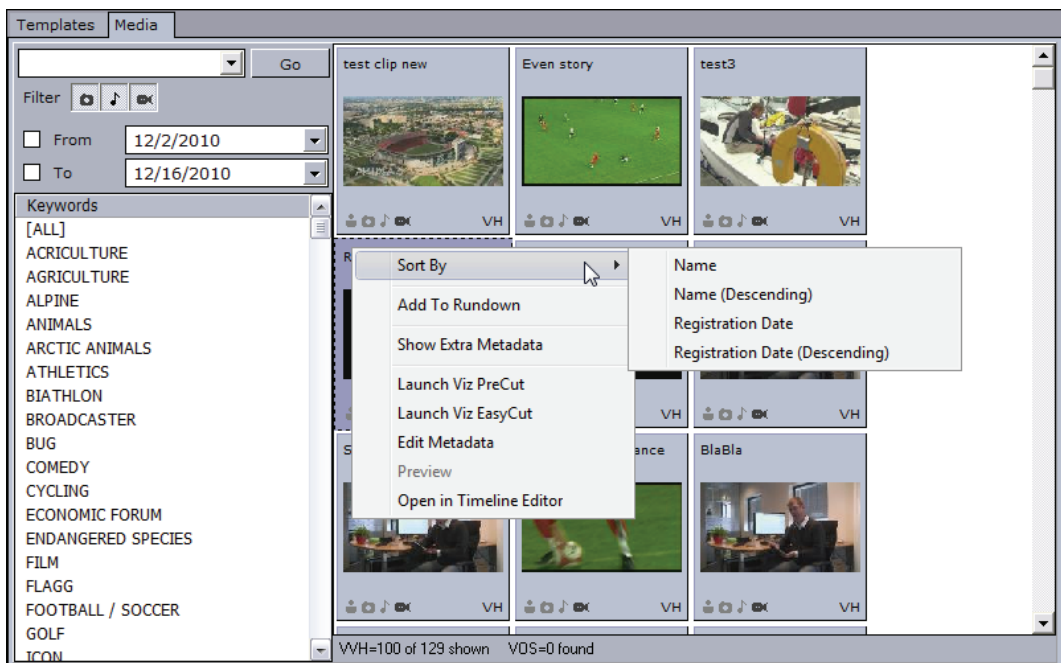
Figure 92: Media
