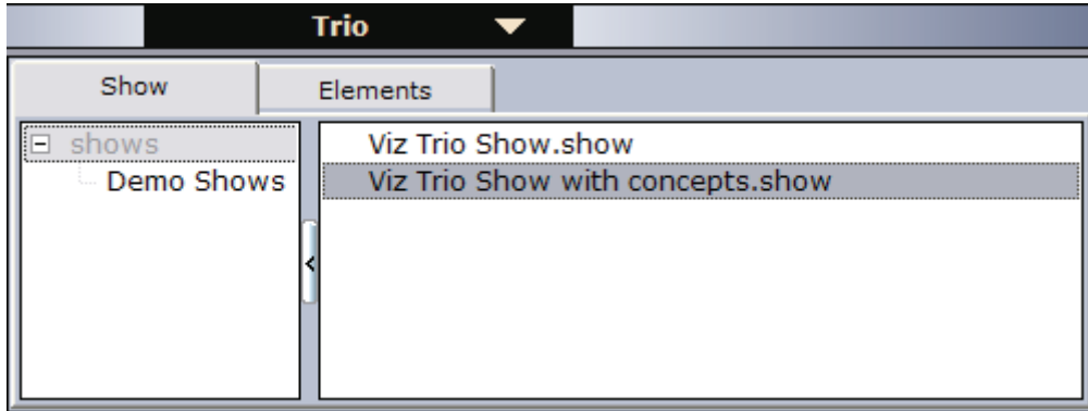
Figure 74: Show view
