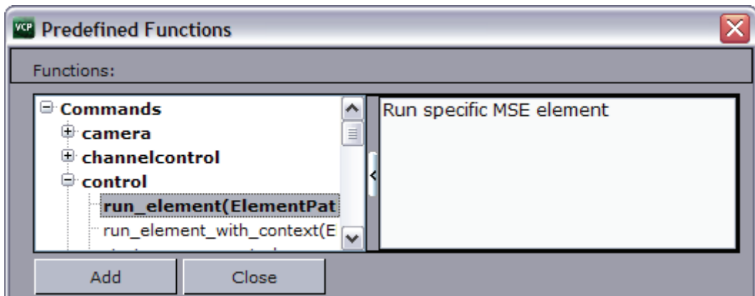
Figure 34: Predefined functions
