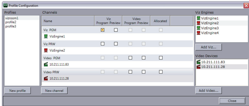
Figure 49: Profile Configuration
