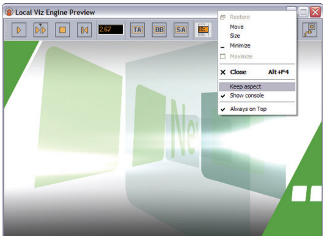
Figure 95: Local preview
