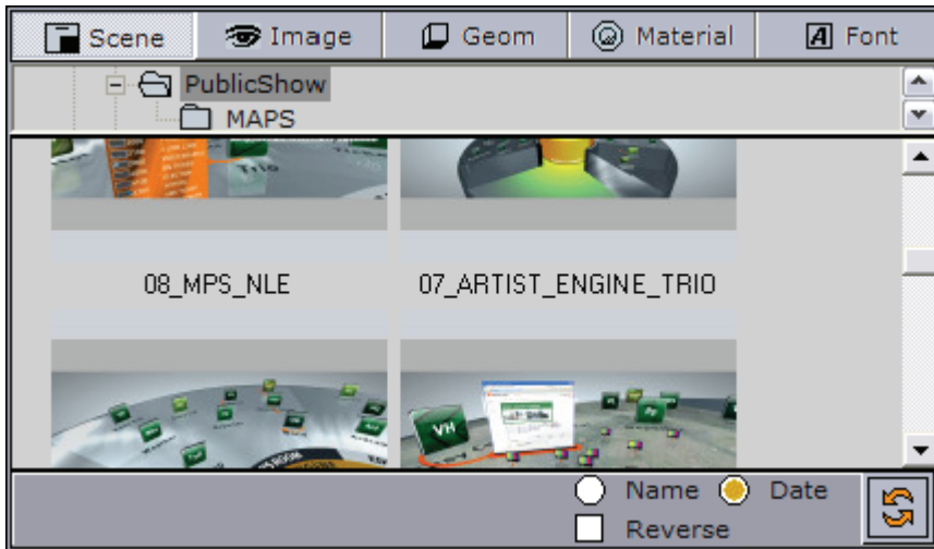
Figure 67: Scenes
