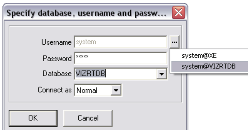
Figure 102: Database login
