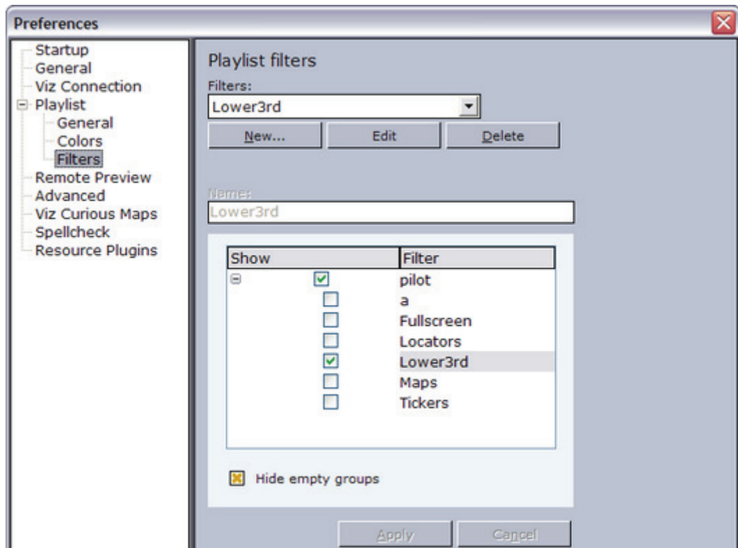
Figure 40: Playlist filters
