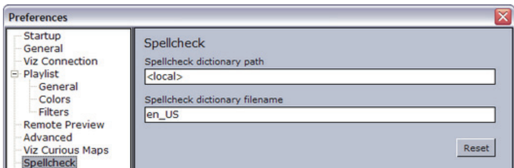
Figure 45: Spell check
