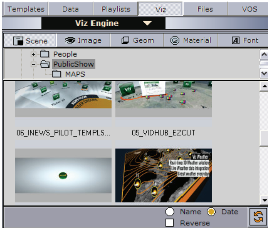
Figure 66: Viz resources
