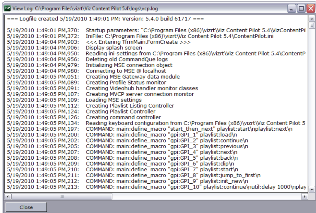
Figure 28: View log
