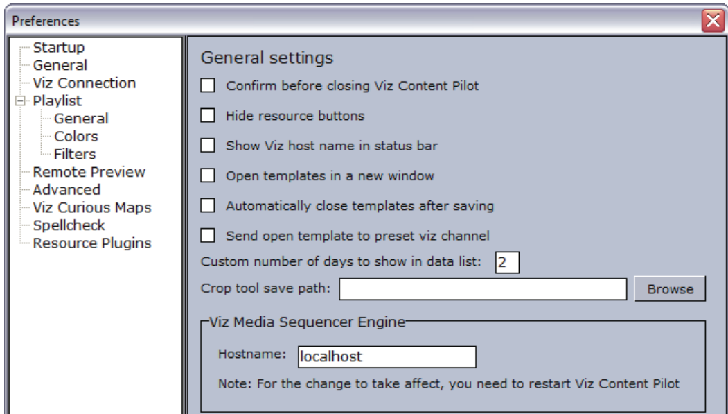
Figure 36: General
