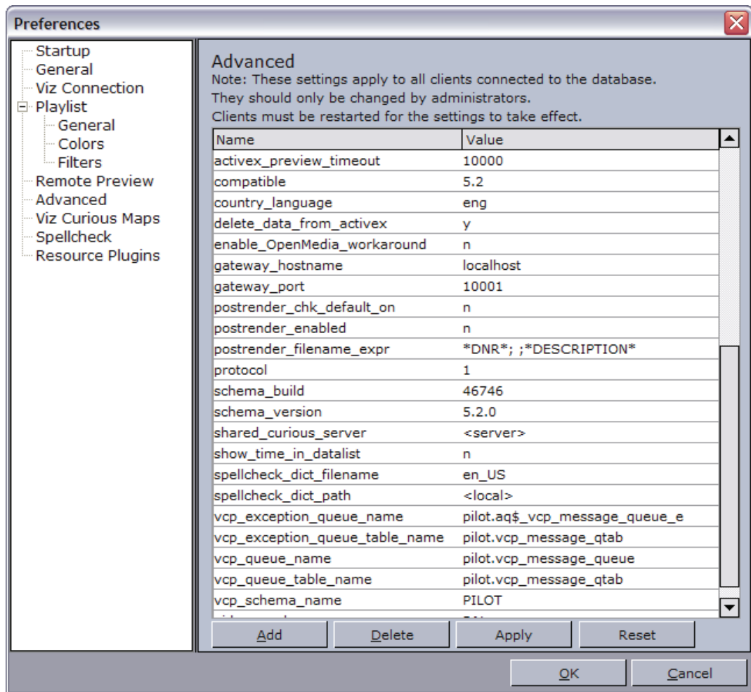
Figure 18: Advanced configuration
