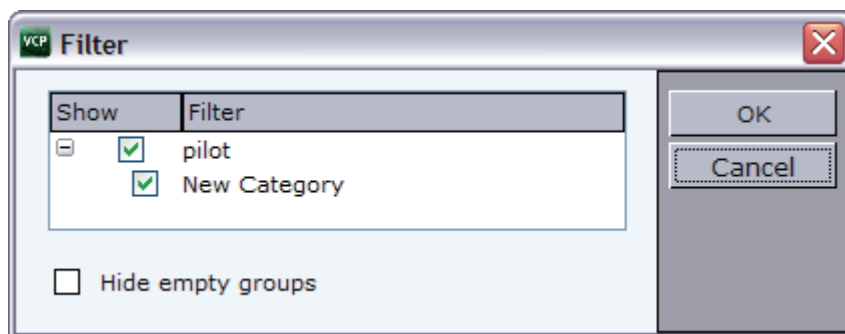
Figure 80: Filter
