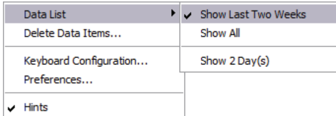
Figure 30: Options menu
