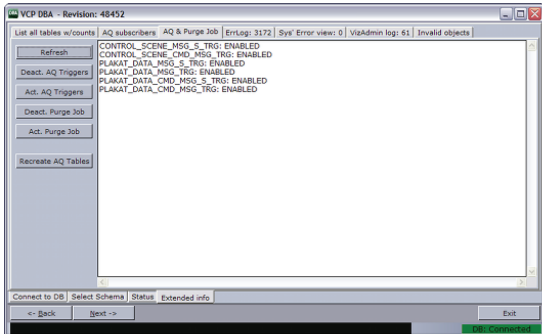
Figure 108: Extended information
