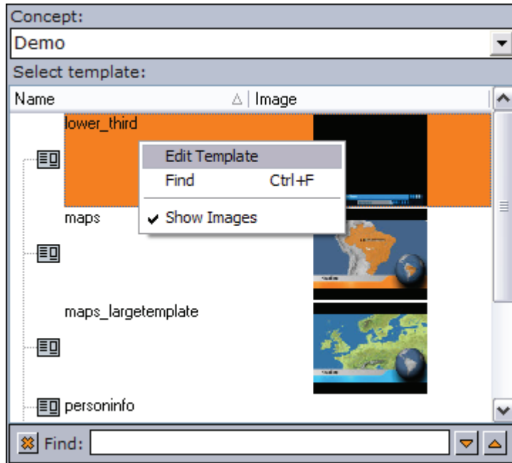
Figure 63: Template resources
