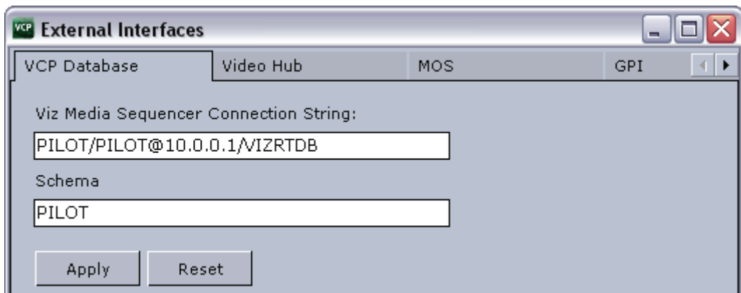
Figure 11: VCP Database
