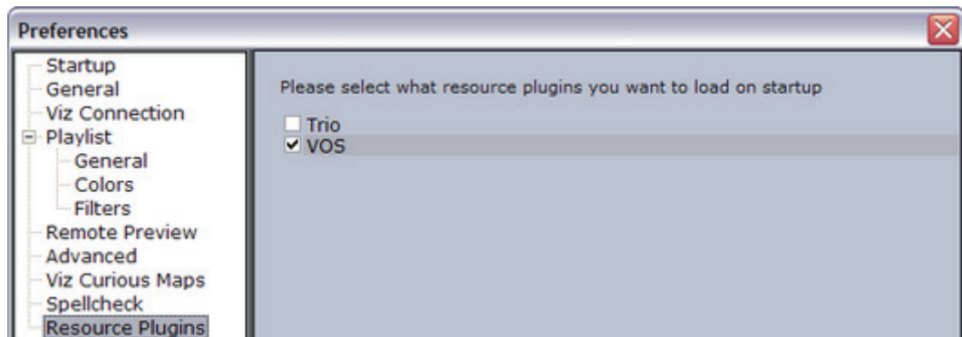
Figure 46: Resource plug-ins
