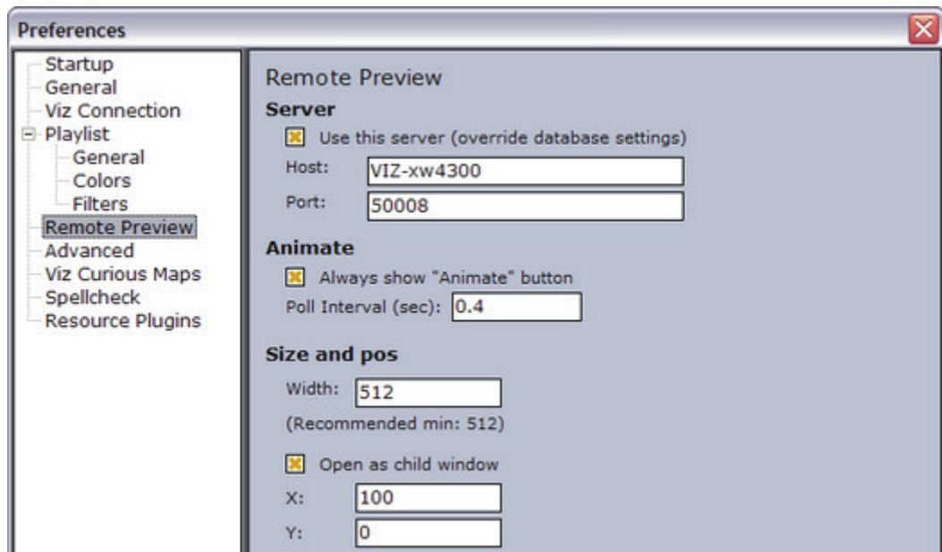
Figure 43: Remote preview
