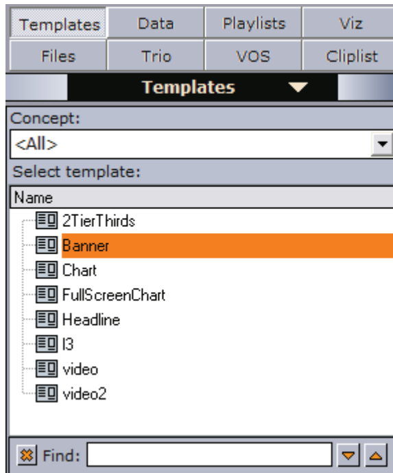
Figure 62: Resource panel
