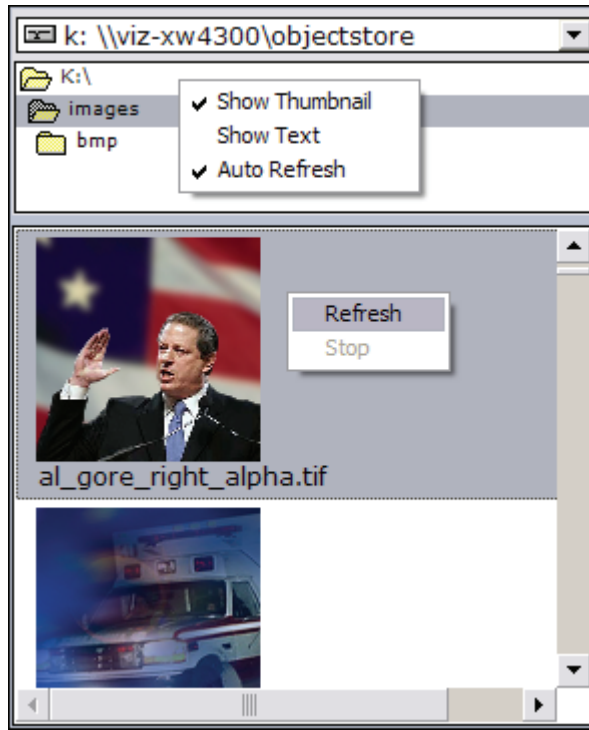
Figure 72: Files
