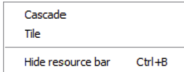
Figure 58: Windows menu
