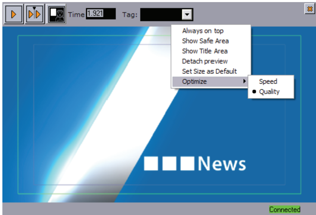
Figure 96: Remote preview
